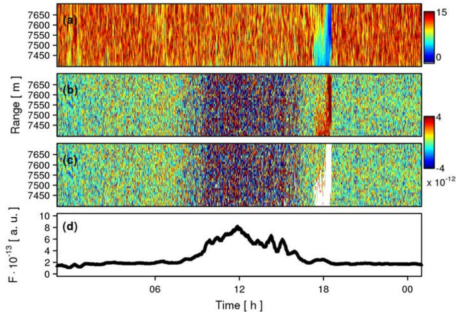
Figure 8. Observations from Vaisala CL31 sensor D (Table 2) at top range gates (7410–7700 m) with cirrus during the early evening on 1 February 2013: (a) relative variance RV (Eq. 14); (b) background-corrected signal \hat{P} ; (c) same as (b) but only including observations with RV > 1; and (d) time series of the noise floor F (Eq. 13) based on the cleaned signal shown in (c) with missing values interpolated linearly.
