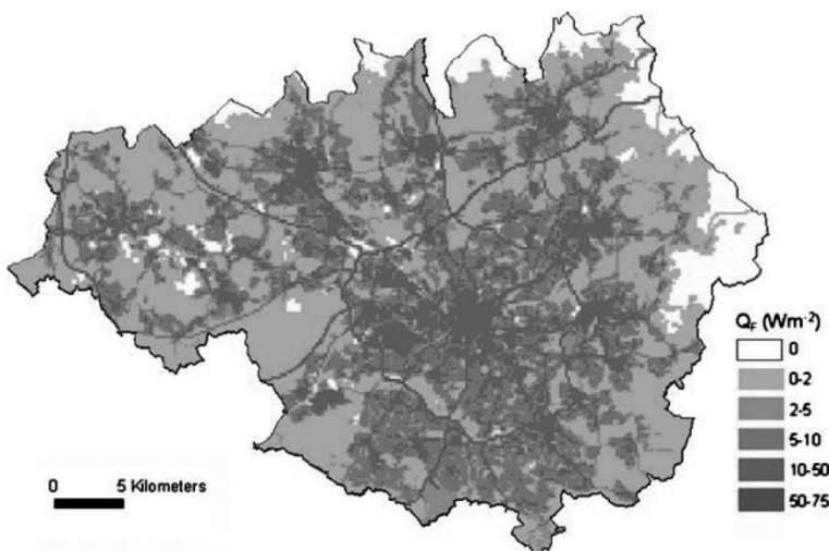
Figure 2. Daily averaged Q_F \text{ (W m}^{-2}\text{)} estimates for Greater Manchester at 200 \text{ m} \times 200 \text{ m} grid, using urban morphology units (source: Smith et al. 2009).
